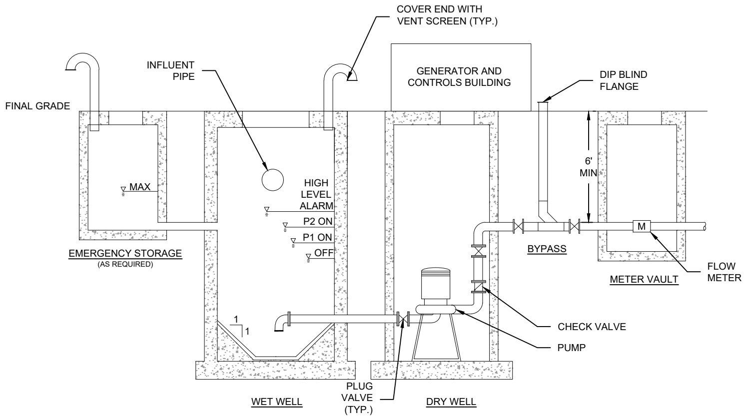
PROFILE VIEW
