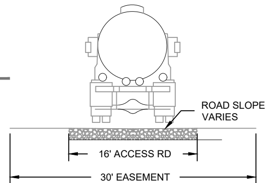
TYPICAL ACCESS ROAD CROSS SECTION
