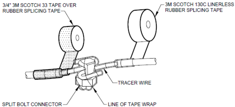
SPLIT BOLT TAPING
