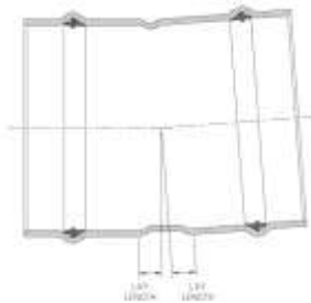
PVC 3 Degree Bend Coupling
