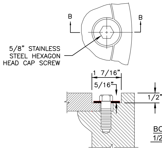
SECTION B-B BOLT INSTALLATION
