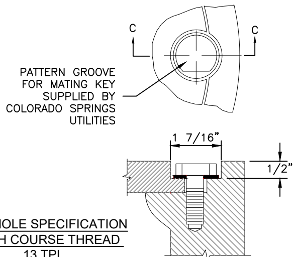
SECTION C-C BOLT INSTALLATION FOR LOCKING COVERS
