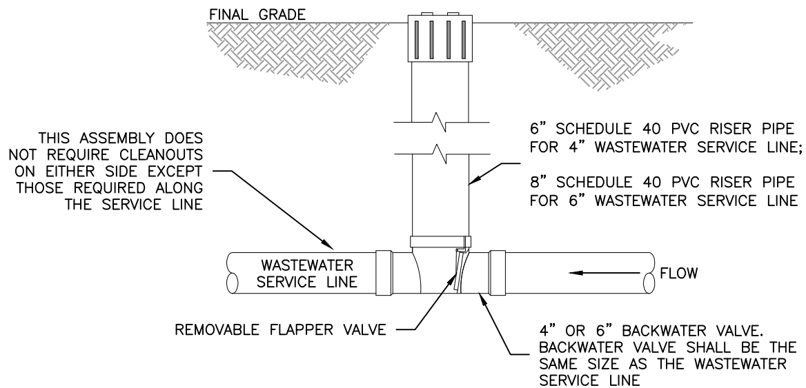
TYPICAL BACKWATER VALVE ASSEMBLY
