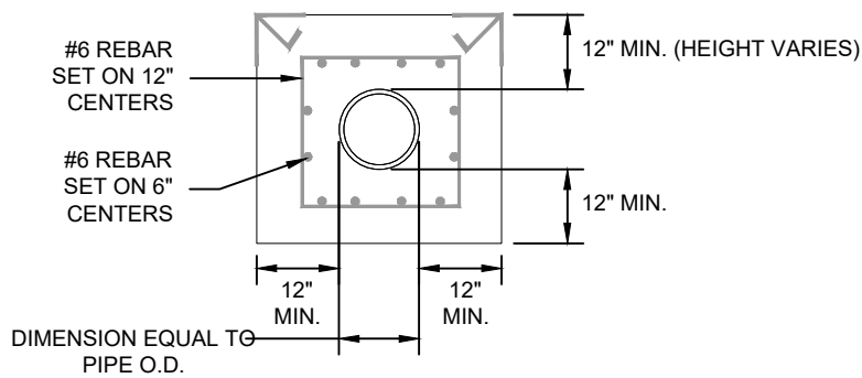
CONCRETE ENCASEMENT DETAIL WITHOUT CAISSON
