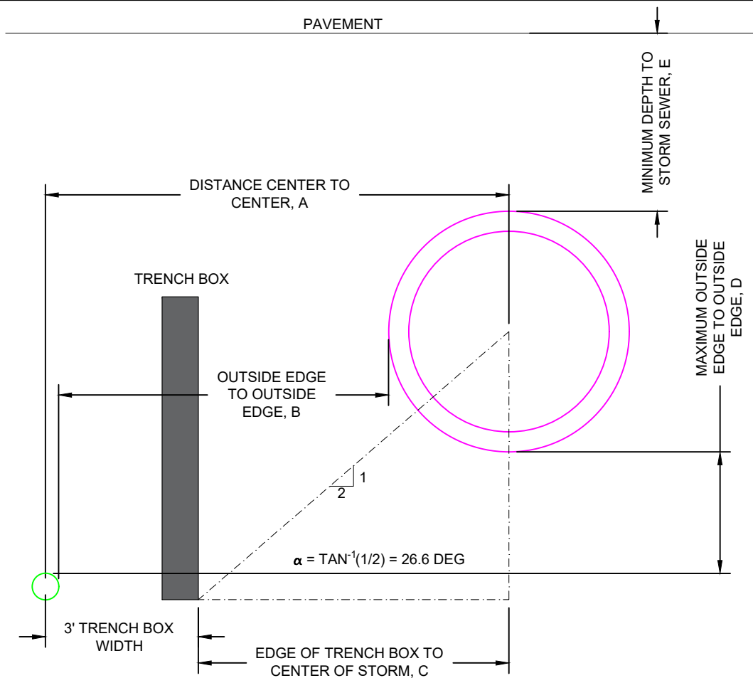
ANGLE OF REPOSE WITH TRENCH BOX FOR REPAIRS AND MAINTENANCE OF WASTEWATER MAIN
