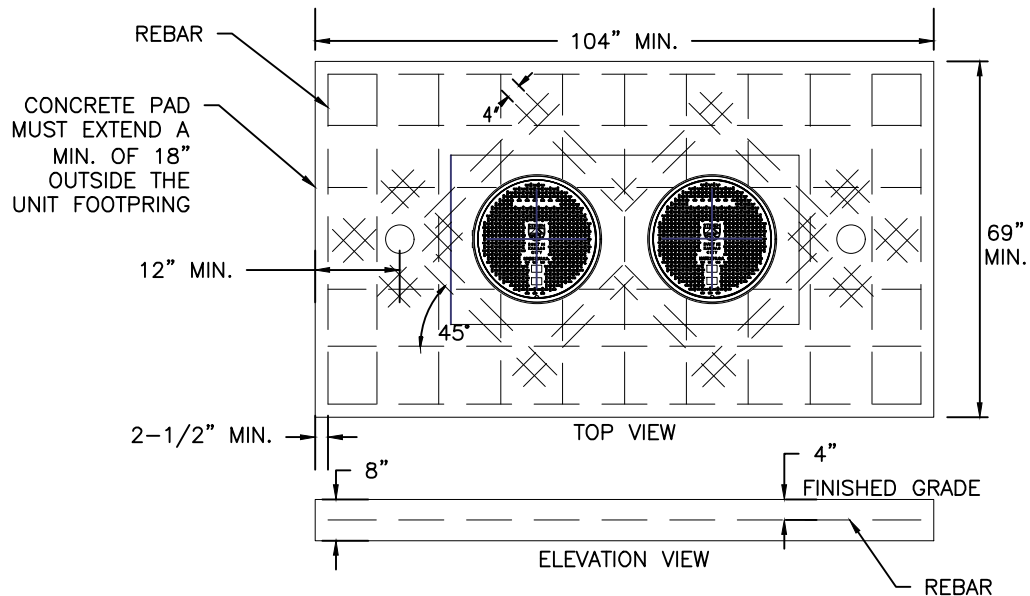
INTERCEPTOR CONCRETE SLAB DETAIL
