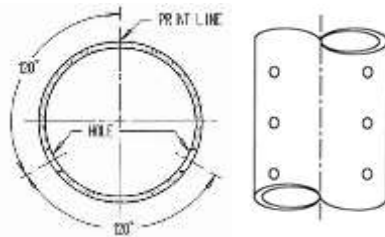
Figure 8-1: Perforated Pipe Hole Configuration
