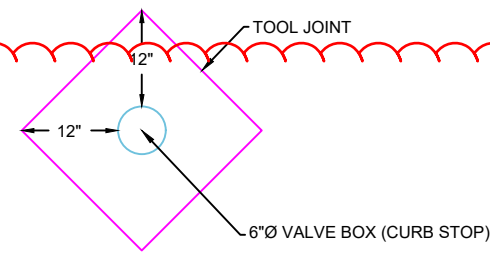
CURB STOP IN DRIVEWAY DETAIL
