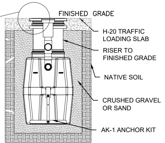
EXCAVATION AND BACKFILL DETAIL
