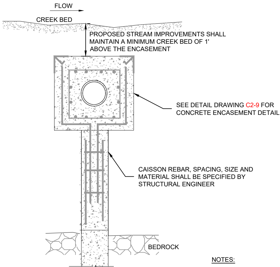
CONCRETE ENCASEMENT DETAIL WITH CAISSON
