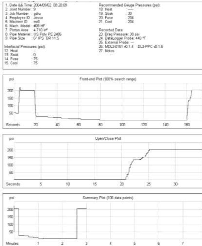
Figure 6-1: Example of a Heat Fusion Joint Record (typical output for a McElroy Data logger)
