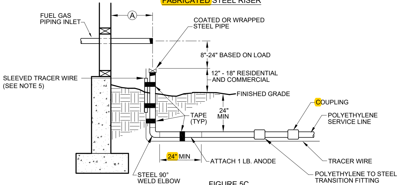
FIGURE 5C SIDE VIEW
