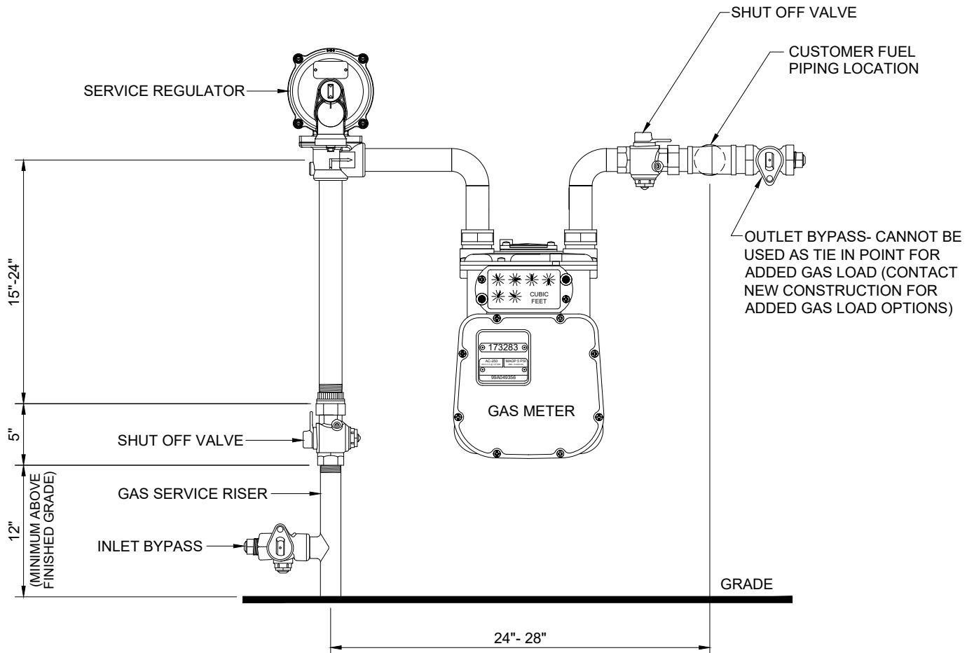
FIGURE 8B TYPICAL COMMERCIAL METER SET 0 - 1,200,000 (BTU/HR)
