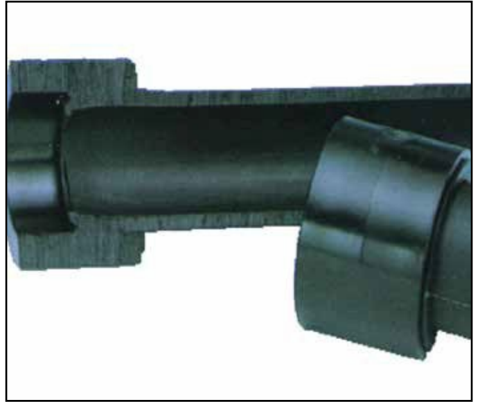
Excessive Stab Depth Caused by Failure to Use a Cold Ring to Use a Cold Ring
