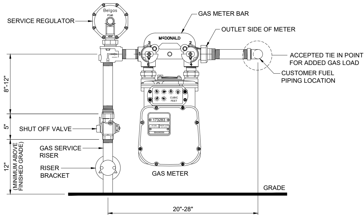
FIGURE 8A TYPICAL RESIDENTIAL METER SET 0 - 1,200,000 (BTU/HR)
