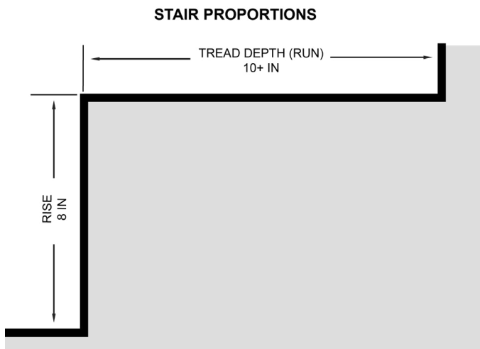
Figure 4–50. Risers range 6–10 in (15–25 cm) and treads are a minimum of 10 inches (25 cm) depending on the trail type and development scale.
