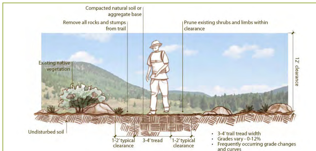
FIGURE 1. TYPICAL TRAIL DIMENSIONS
