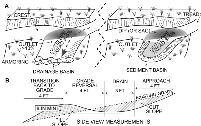
Figure 4–2. A properly constructed rolling dip can be a sustainable solution for a poorly designed or constructed trail. The side view measurements in the lower diagram are estimates from a hand-built hiking trail. Dimensions will change depending on user type, trail grade, soil condition, prevailing hillside slope, and typical rainfall patterns. Diagrams based on Forest Service standard trail drawings STD 927–01 and 927–02.
