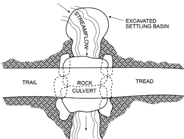
Figure 4–17. Settling basin on the upstream side of the culvert to prevent the culvert from clogging with silt and debris. Diagram based on Forest Service standard trail drawing STD 921–30–01.
