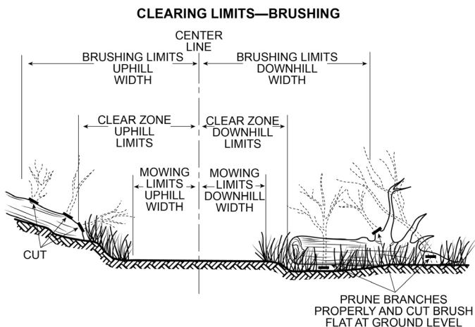
Figure 3–5. The trail corridor clearing dimensions change depending on the trail type and development scale. The clearing dimensions for each trail are documented in the TMO. Diagram based on Forest Service standard trail drawing STD 912–02.
