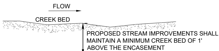
TYPICAL STREAM CROSSING CROSS SECTION
