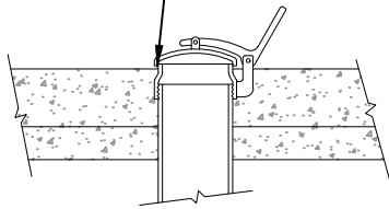
POUR TO LIP OF HATCH TO ALLOW EASY WASH-DOWN OF CONCRETE PAD
