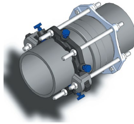
Sigma One Lok Series SLDEH for DIP (3" – 8" @ 350 psi, 10"- 16" @ 300 psi, 18" – 36" @ 200 psi)
