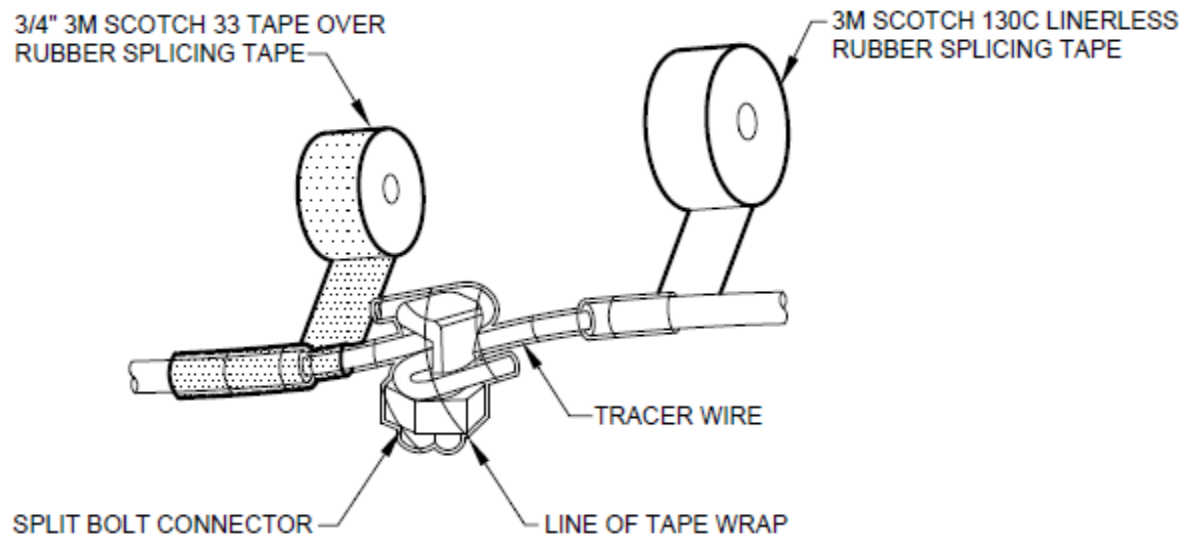
SPLIT BOLT TAPING
