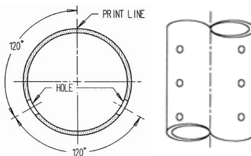
Figure 8-1: Perforated Pipe Hole Configuration
