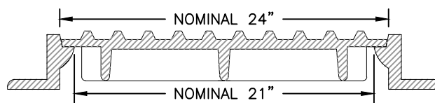
SECTION A-A COVER SECTION
